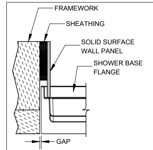
WALL PANEL INSTALL DETAIL
