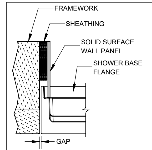
WALL PANEL INSTALL DETAIL
