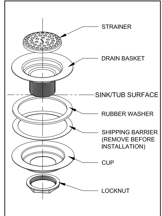
Drain Assembly #320001
