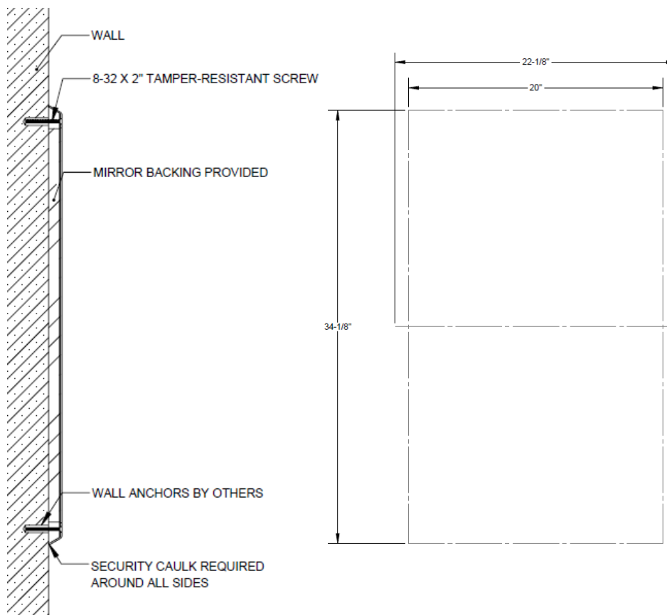
Mounting anchor locations
