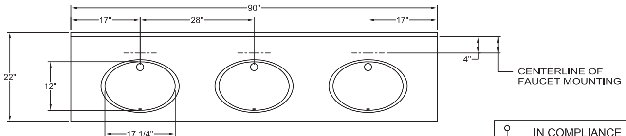
PLAN VIEW
