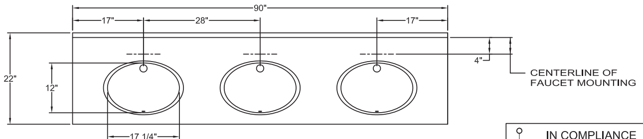
PLAN VIEW
